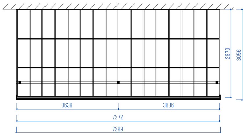
TF1MA-C-24.10C-L (12.10+12.10 Connect)
